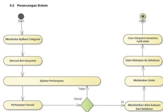
Gambar 1. Gambar Flowchart System
